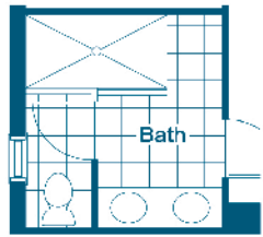
Master Bath Double Sink Option
