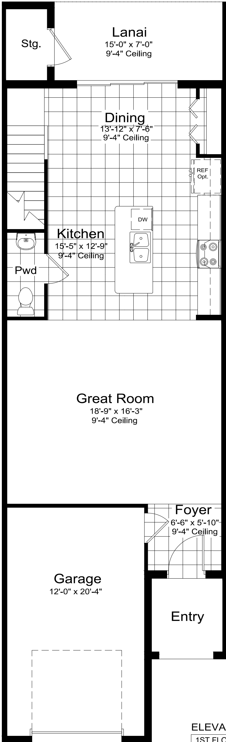
First Floor
