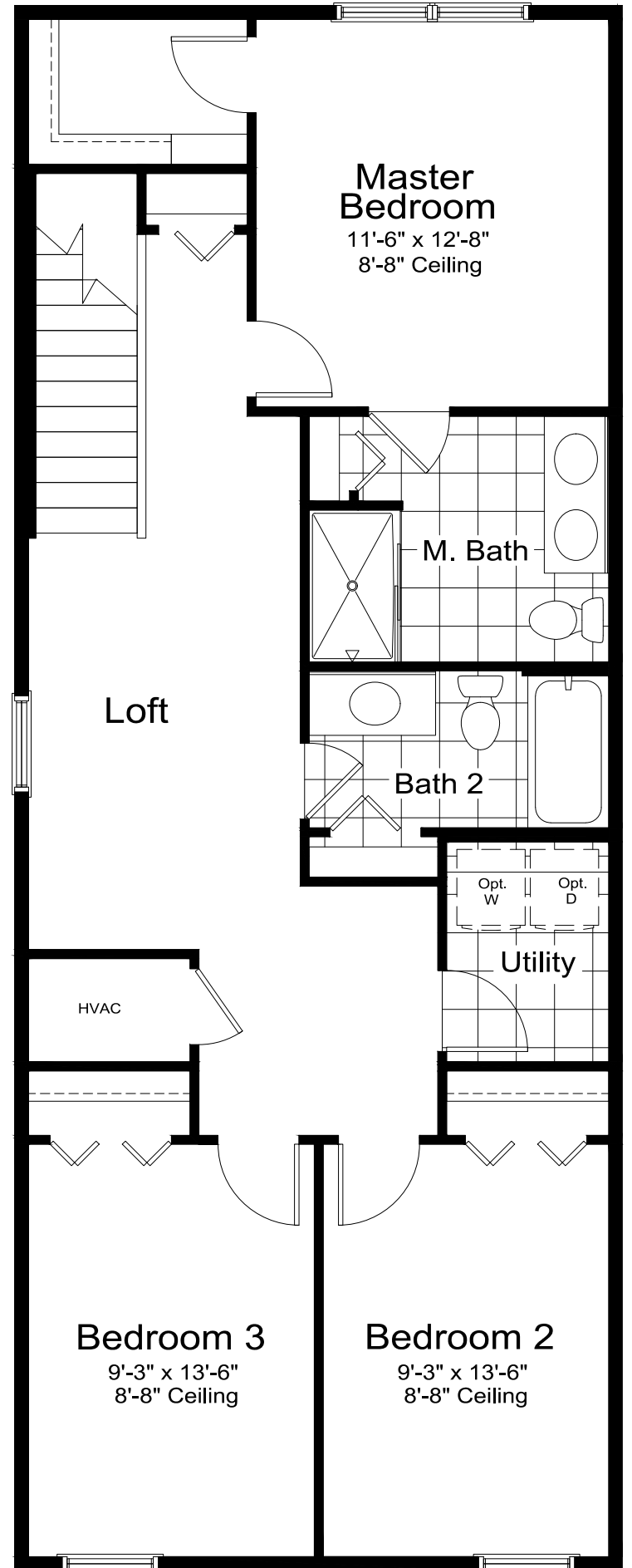
Second Floor
